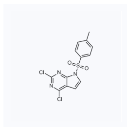
1048296 现货 CAS: 934524-10-4
