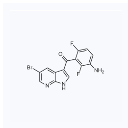
1061870 现货 CAS: 1312941-98-2
