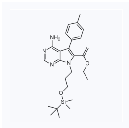
1059488 现货 CAS: 821794-86-9
