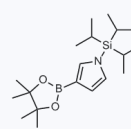
1122299 CAS: 365564-11-0
