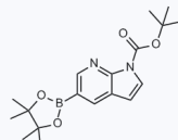
1126610 CAS: 1370616-23-1
