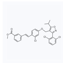
1058752 CAS: 933799-50-9
