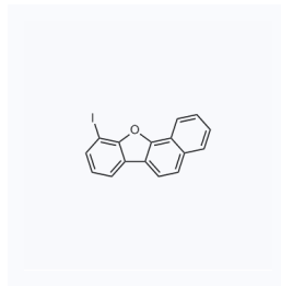
1170934 CAS: 2271091-82-6
