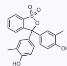
1079955 CAS: 1733-12-6
