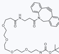
1178624 CAS: 1255942-12-1
