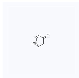
1122680 CAS: 1514112-02-7
