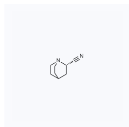
1070201 CAS: 885517-04-4
