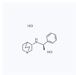
1019226 CAS: 128311-06-8
