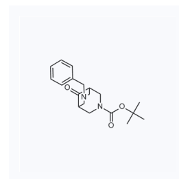
1051255 CAS: 227940-70-7
