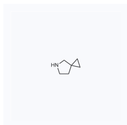
1127956 CAS: 185-50-2
