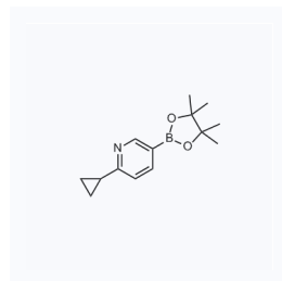
1064846 现货 CAS: 893567-09-4
