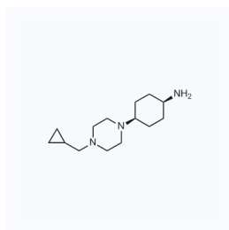
1057890 现货 CAS: 755039-90-8
