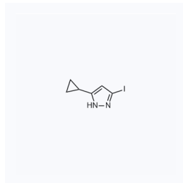
1171787 现货 CAS: 1218791-06-0
