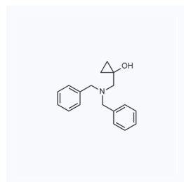
1107493 现货 CAS: 428855-17-8
