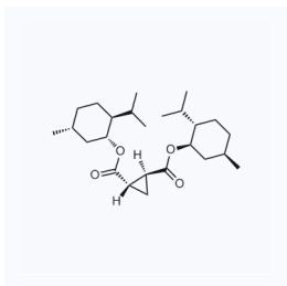
1058536 现货 CAS: 96149-00-7
