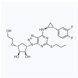
1060015 现货 CAS: 2096989-55-6
