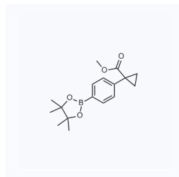
1061926 现货 CAS: 1396007-85-4
