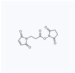
1035871 现货 CAS: 55750-62-4
