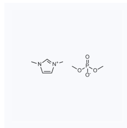
1039177 CAS: 654058-04-5
