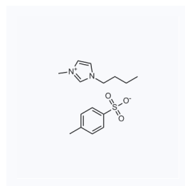
1032220 CAS: 410522-18-8
