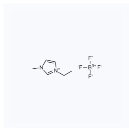
1021391 现货 CAS: 143314-16-3
