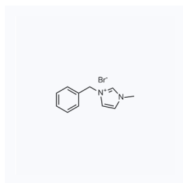
1203325 CAS: 65039-11-4
