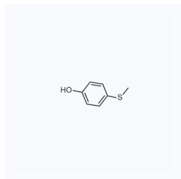
1016112 现货 CAS: 1073-72-9
