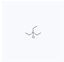
1169916 现货 CAS: 994-30-9
