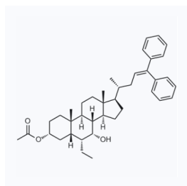
1191013 CAS: 1605309-10-1
