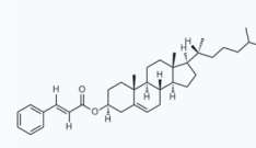
1025042 CAS: 1990-11-0
