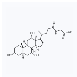
1033302 现货 CAS: 475-31-0
