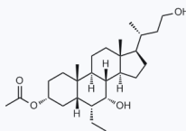
1191015 CAS: 1605309-13-4
