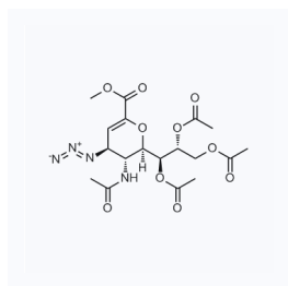
1151917 现货 CAS: 130525-58-5
