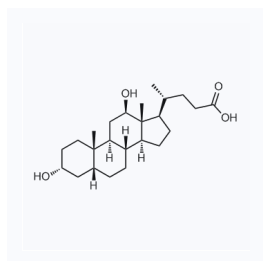
1150757 现货 CAS: 570-62-7
