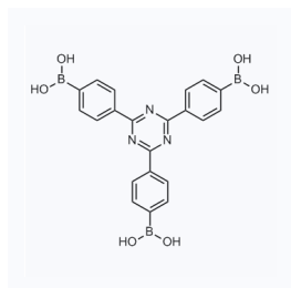
1181841 CAS: 910231-21-9
