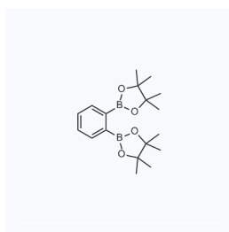
1061927 现货 CAS: 269410-07-3
