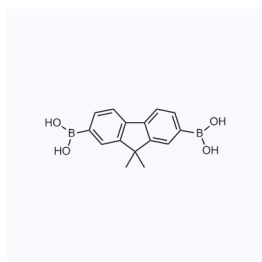
1050792 现货 CAS: 866100-14-3
