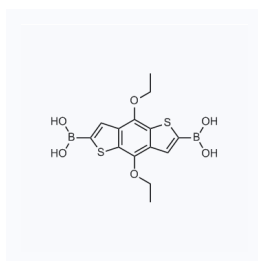
1181782 CAS: 2023811-72-3
