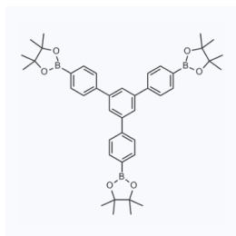
1181119 CAS: 1017967-97-3
