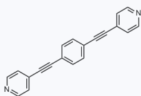
1181041 CAS: 158525-01-0
