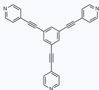
1181024 CAS: 168289-78-9
