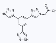
1180699 CAS: 958299-25-7
