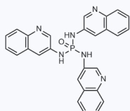
1181950 CAS: 2097565-50-7
