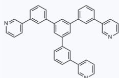
1133412 CAS: 921205-03-0
