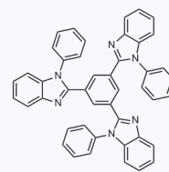
1106687 CAS: 192198-85-9
