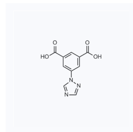
1181180 CAS: 2241598-39-8
