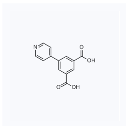
1180712 CAS: 1262962-06-0
