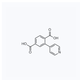
1181112 CAS: 1238617-40-7
