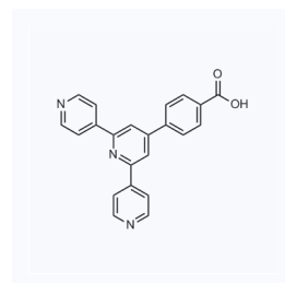
1181549 CAS: 1370206-12-4
