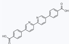
1181558 CAS: 1373759-05-7
