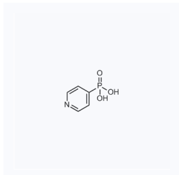
1181739 CAS: 58816-01-6
