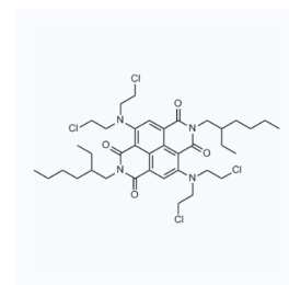
1181633 CAS: 2043039-67-2
