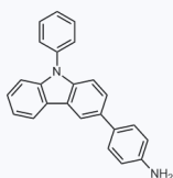
1216995 CAS: 1370034-59-5
