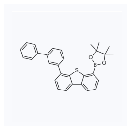
1206500 CAS: 1858289-64-1
