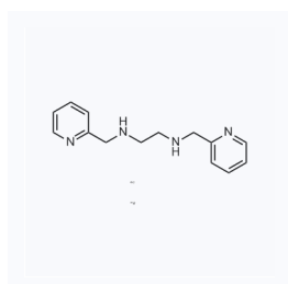
1156149 CAS: 1310544-60-5
