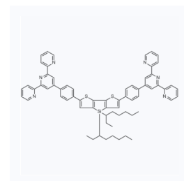
1182180 CAS: 1800104-25-9
