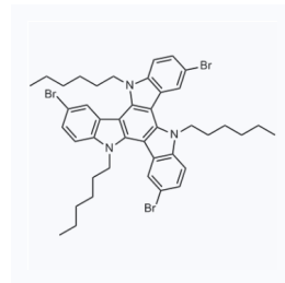
1169534 CAS: 862856-06-2
