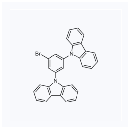
1130530 CAS: 750573-24-1
