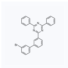
1206505 CAS: 1606981-69-4
