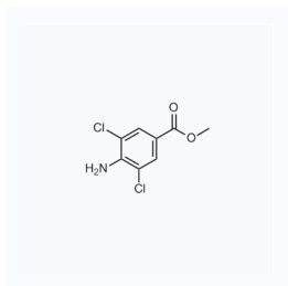
1069645 现货 CAS: 41727-48-4
