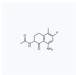
1110876 现货 CAS: 182182-31-6
