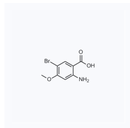
1112123 现货 CAS: 169045-04-9
