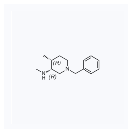
1033348 现货 CAS: 477600-70-7
