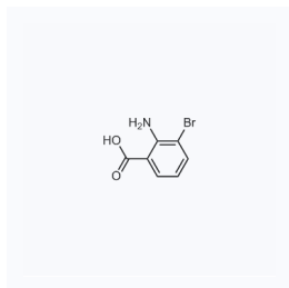
1025568 现货 CAS: 20776-51-6
