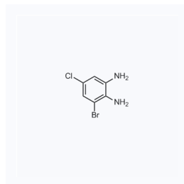
1061937 现货 CAS: 500862-39-5
