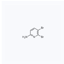
1063136 现货 CAS: 89284-11-7
