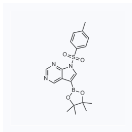
1120782 CAS: 934178-97-9
