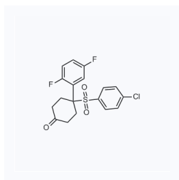
1057248 CAS: 471903-20-5
