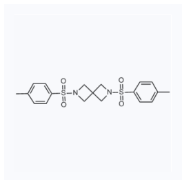
1070794 CAS: 13595-48-7
