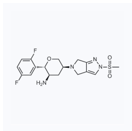
1127021 CAS: 1443380-88-8
