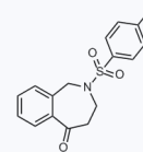
1047896 CAS: 1951439-55-6
