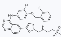
1171057 CAS: 1393112-45-2
