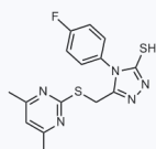
1141226 CAS: 887205-52-9
