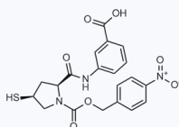
1089752 CAS: 202467-69-4
