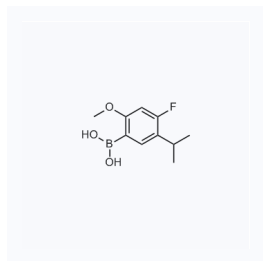
1059486 现货 CAS: 875446-29-0
