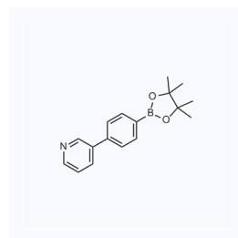
1068376 现货 CAS: 929203-04-3
