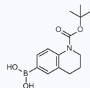
1180560 CAS: 1260150-04-6
