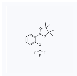
1151783 现货 CAS: 832114-04-2
