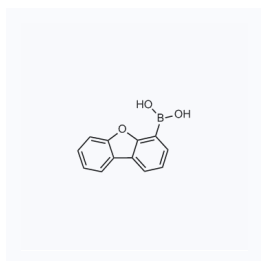
1014497 现货 CAS: 100124-06-9
