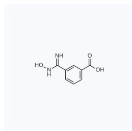
1059864 现货 CAS: 199447-10-4
