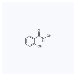
1045849 现货 CAS: 89-73-6
