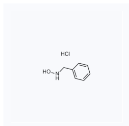
1028612 现货 CAS: 29601-98-7
