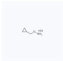
1066034 现货 CAS: 74124-04-2
