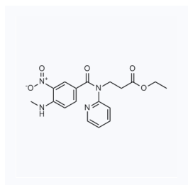
1059241 CAS: 429659-01-8
