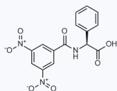
1202203 现货 CAS: 90761-62-9
