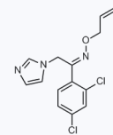
1198121 CAS: 928209-03-4
