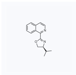
1158175 现货 CAS: 1701405-00-6
