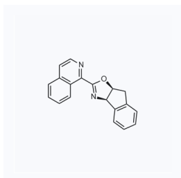
1215745 现货 CAS: 2126902-95-0
