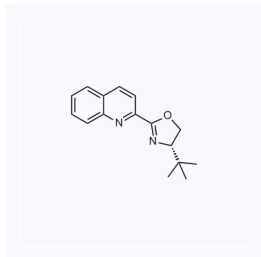
1158943 现货 CAS: 226387-12-8
