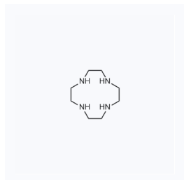
1028598 CAS: 294-90-6
