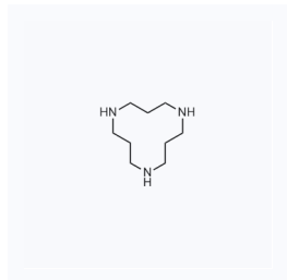
1091929 CAS: 294-80-4
