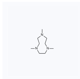
1114409 CAS: 96556-05-7
