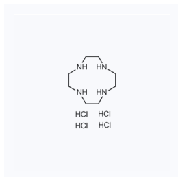
1155710 CAS: 10045-25-7
