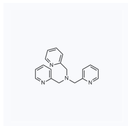
1156307 CAS: 16858-01-8
