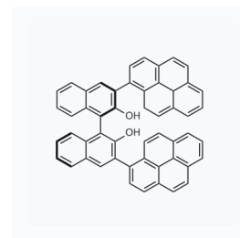
1212247 CAS: 1854074-51-3
