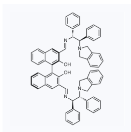
1155767 CAS: 1620285-48-4
