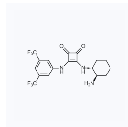
1174954 CAS: 1888443-73-9
