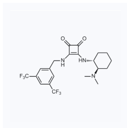
1163862 CAS: 1449676-73-6
