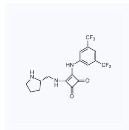
1163798 CAS: 1356935-80-2
