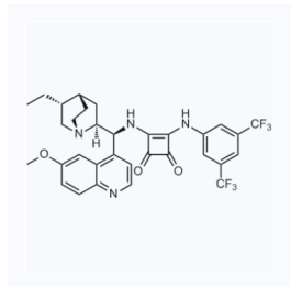
1163792 现货 CAS: 1352957-59-5
