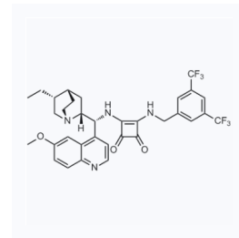
1163806 现货 CAS: 1363811-07-7
