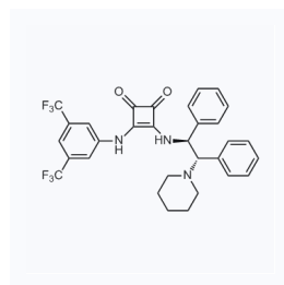
1175531 现货 CAS: 1943732-17-9
