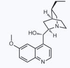
1021825 CAS: 1476-98-8
