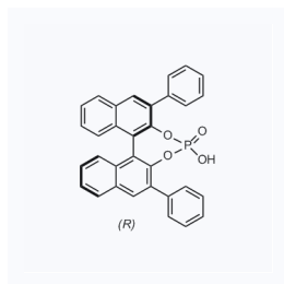
1155176 现货 CAS: 695162-86-8
