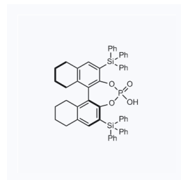
1163542 现货 CAS: 1157989-25-7
