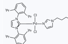
1161585 CAS: 1537173-01-5
