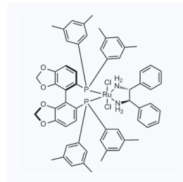
1152741 CAS: 944450-45-7
