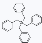
1182082 CAS: 24356-01-2
