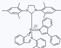
1155666 CAS: 934538-12-2
