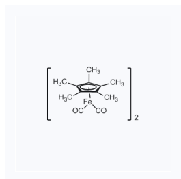
1177311 CAS: 35344-11-7
