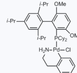
1105791 现货 CAS: 1148148-01-9
