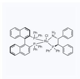
1152934 CAS: 1150112-53-0
