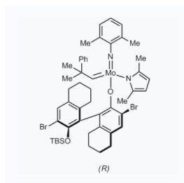
1182476 CAS: 1887760-68-0
