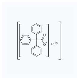
1152538 CAS: 142214-04-8
