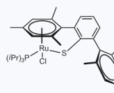
1155207 CAS: 1621182-04-4
