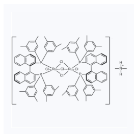
1047118 CAS: 944451-08-5
