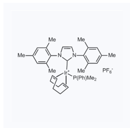
1153478 CAS: 1019853-03-2
