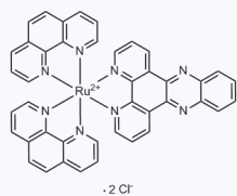
1182005 CAS: 132045-66-0
