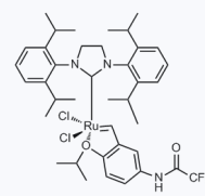
1151943 CAS: 1212008-99-5
