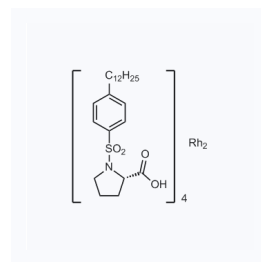
1152553 CAS: 178879-60-2
