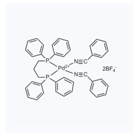
1105875 CAS: 175079-12-6
