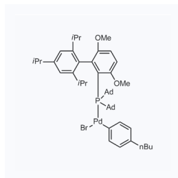
1154542 CAS: 1415050-56-4
