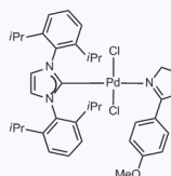
1161592 CAS: 1586000-51-2
