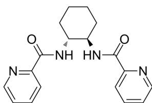
Relative stereochemistry
