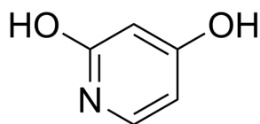
Pyridine-2,4-diol
