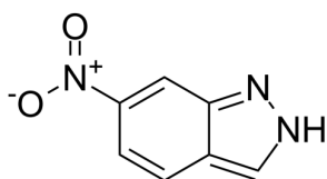
6-Nitro-2H-indazole
