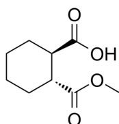
Relative stereochemistry
