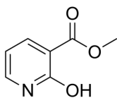
Methyl 2-hydroxynicotinate
