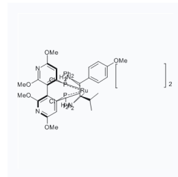
1284475 CAS: 1036379-67-5
