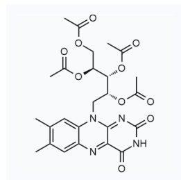
1509524 CAS: 2356187-82-9
