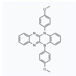
1509510 CAS: 2361129-08-8
