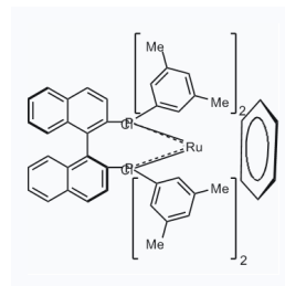
1284481 CAS: 1229001-09-5
