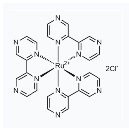
1155627 现货 CAS: 80925-50-4
