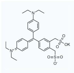
1284463 CAS: 93942-43-9
