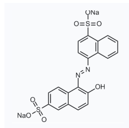
1284509 CAS: 2302-96-7
