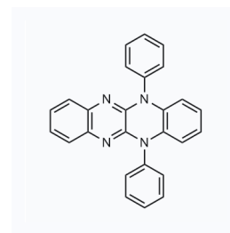
1509516 CAS: 2361129-09-9
